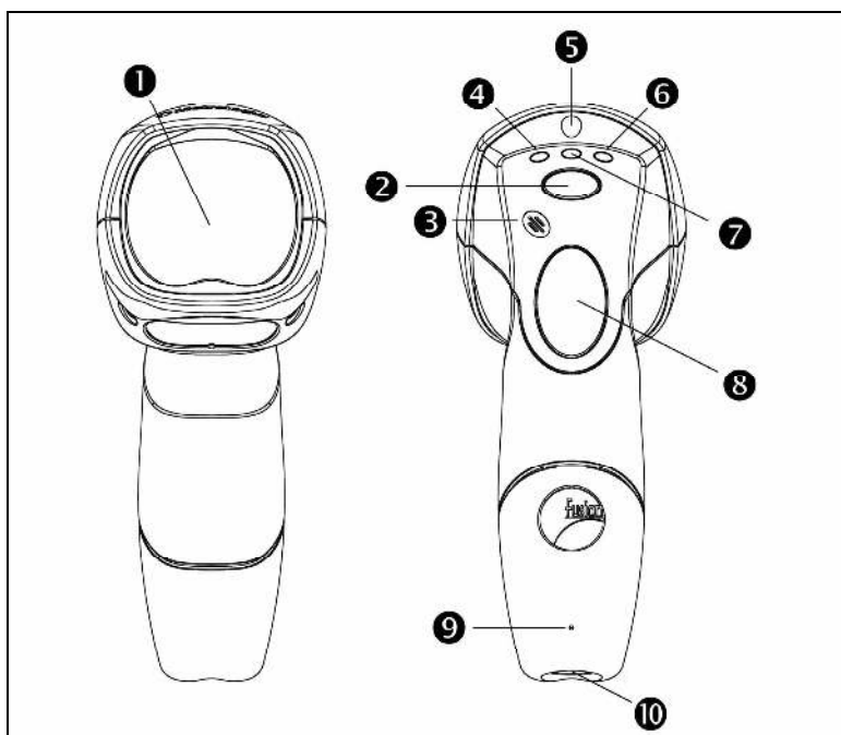
Figure 1. Scanner Components
