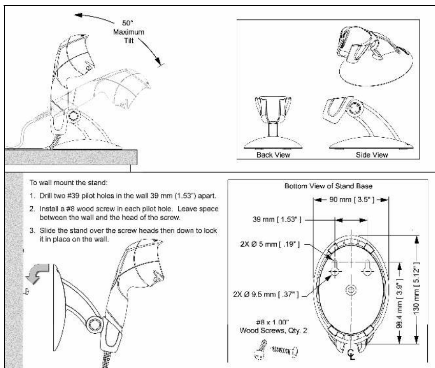
Figure 3. Stand Specifications
